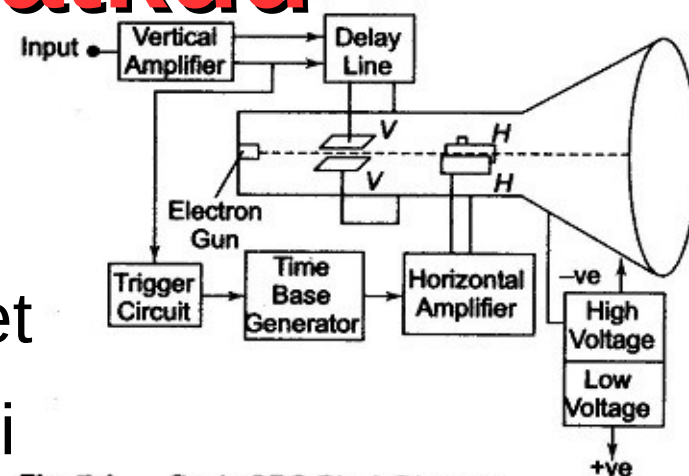
Fig. 7.4 Basic CRO Block Diagram
